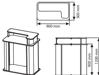
Rectangular Ledge Promostand
