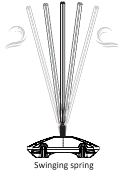
Swinging spring
