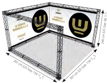
Model 771 / UCT15BM771 Truss U-Shape 4 x 4
