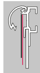
0.59" / 15 mm Profile
