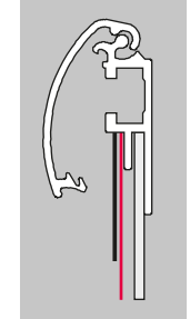
1" / 25 mm Profile
