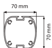
Free Standing Profile, 2 channel 70x70 mm
