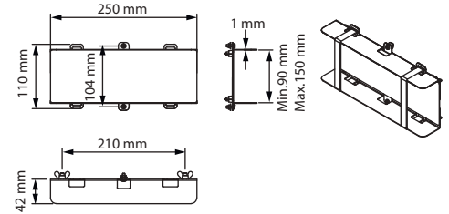
Box Bracket
