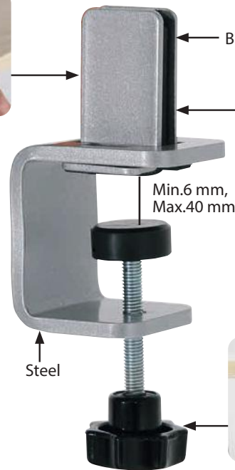
Panel gripper
