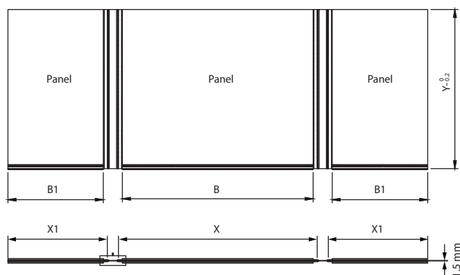
Panel with slot
