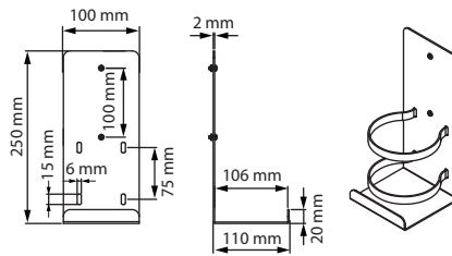
Pump Bracket
