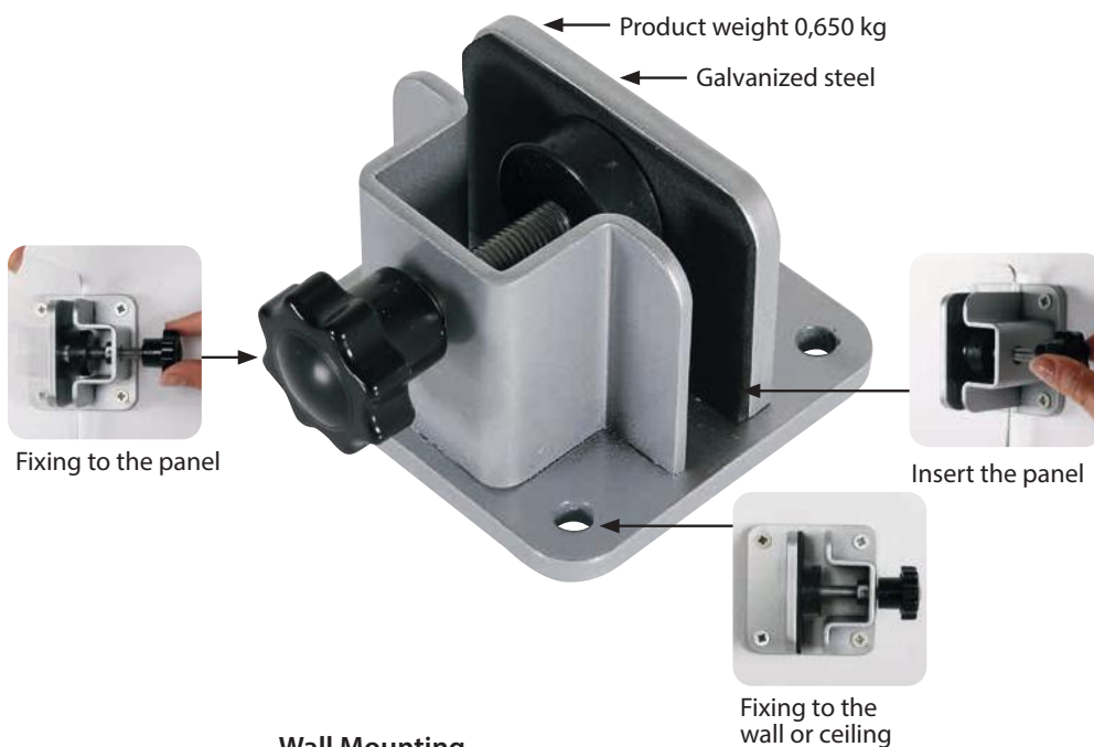
Wall Mounting
