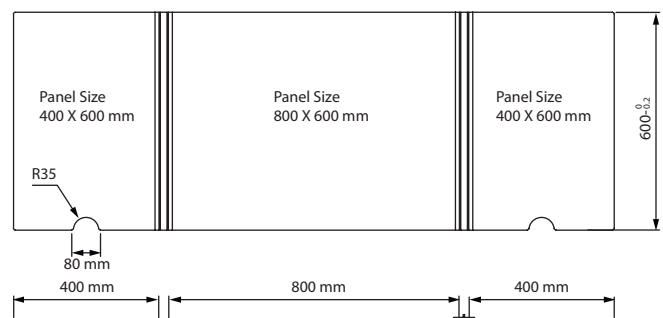
Panel with cable outlet
