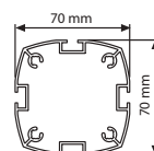
Free Standing Profile, 4 channel 70x70 mm
