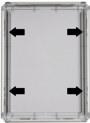
Screw & anchor mounting
