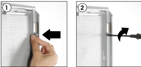
Hanger mounting
