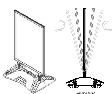
Swinging spring
