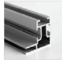
Profile / UYUP014102 Single Sided Maxi profile. Dame Frame Profile. 3 meters. 34x32 mm. Profil / UYUP014102 Single Sided Maxi Profil. Dame Frame Profil. 3 meter. 34x32 mm.
