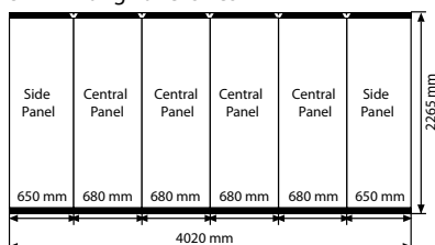
3x4 Printing Panel Sizes
