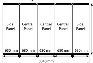
3x3 Printing Panel Sizes
