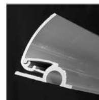
Profile / UYUP011000 Aluminium Poster Clamp profile. Top and bottom profiles are silver anodized.
